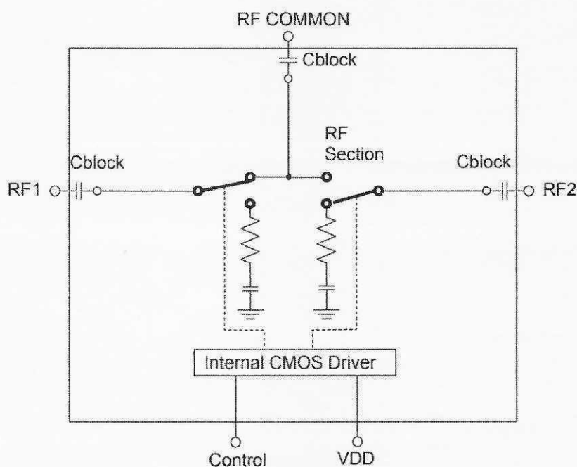
Figure 1: Schematic and Application Circuit
